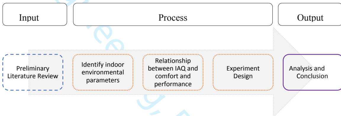
Figure 1: Methodology flowchart
