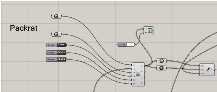
Figure 23: PackRat Definition
