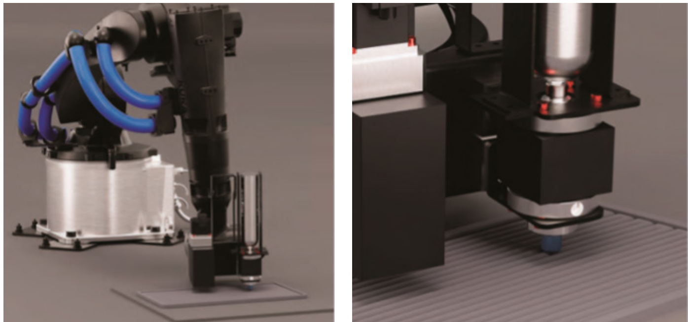
Figure 22: Robotic Simulation of Pattern A
