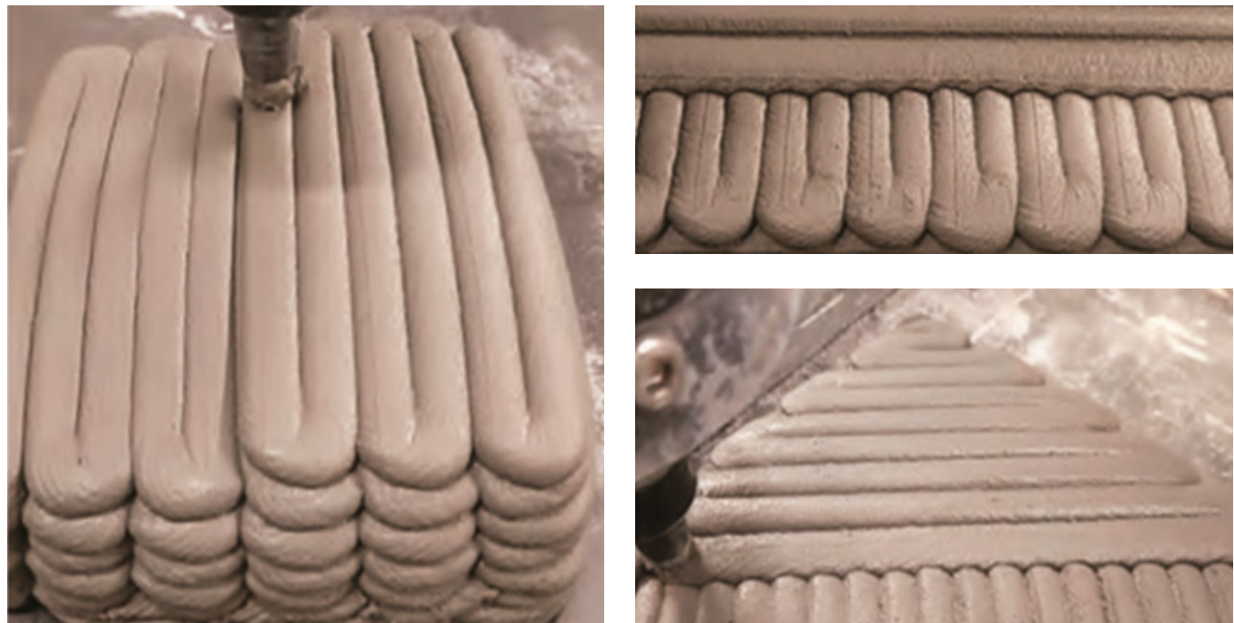
Figure 21: Printing Process Pattern A
